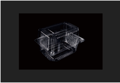
型号: JM-01 装箱: 2400个 材质: PET 尺寸: (外) 135mm*110mm*87mm (内) 124mm*97mm*85mm
